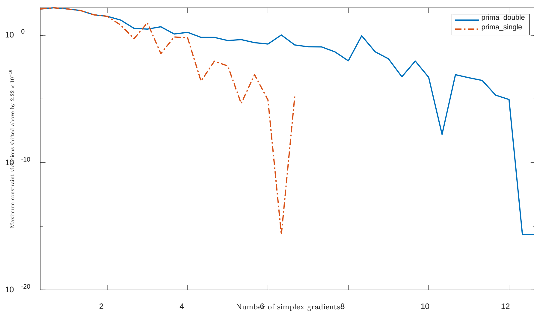
Solving "HS19" with "plain" feature
