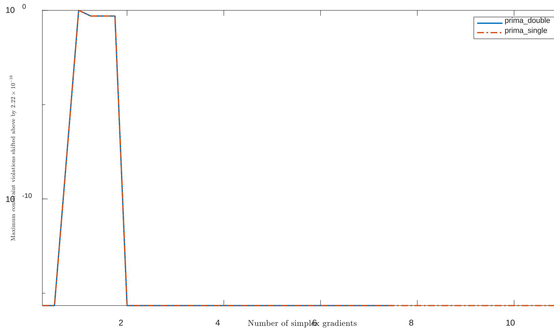
Solving "HS35" with "plain" feature
