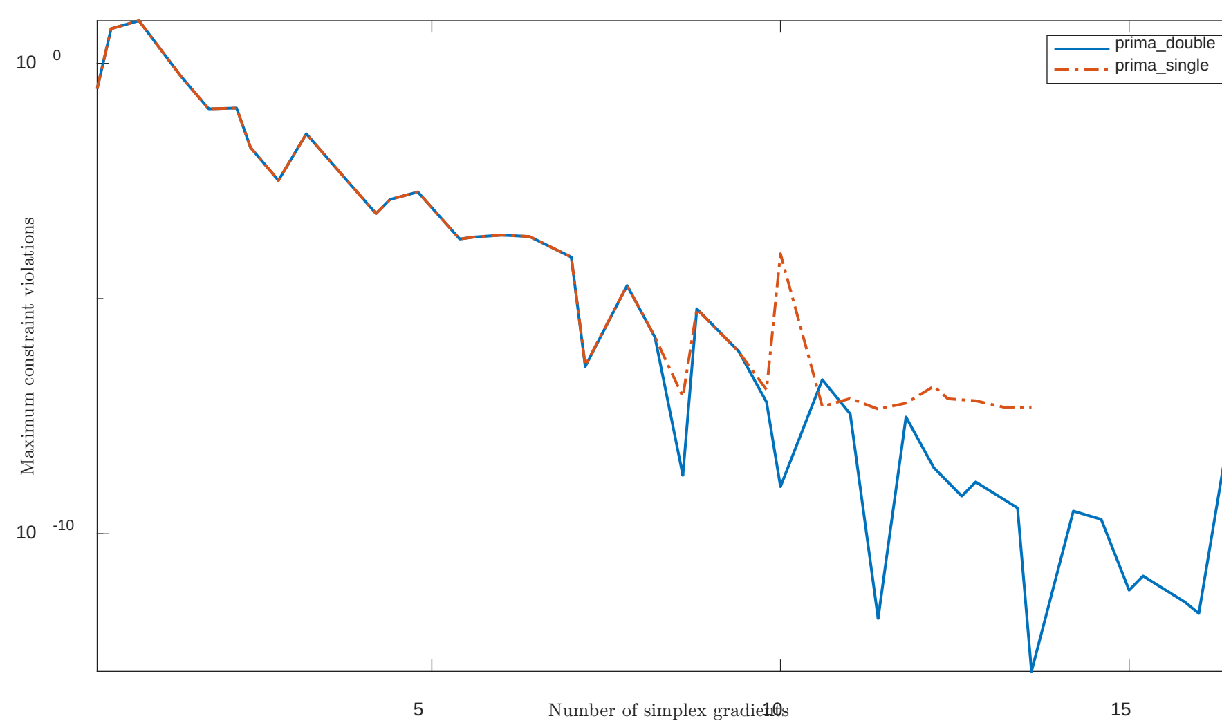
Solving "HS40" with "plain" feature
