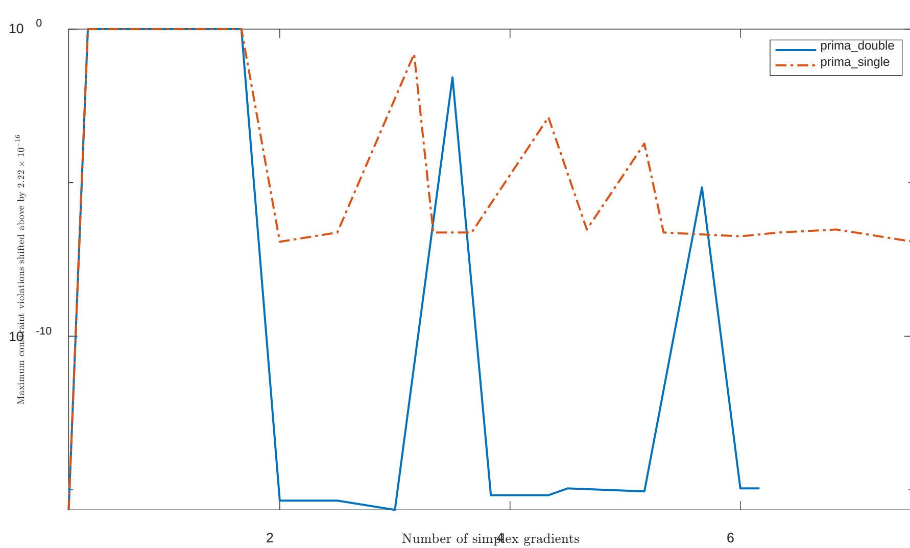
Solving "HS51" with "plain" feature
