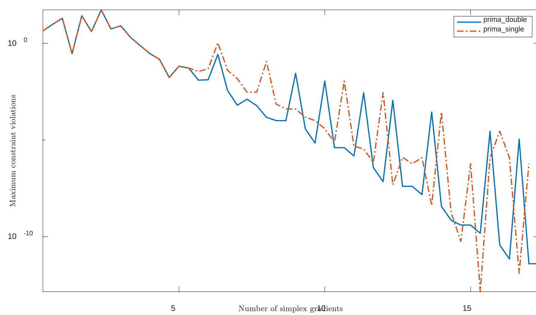
Solving "HS6" with "plain" feature
