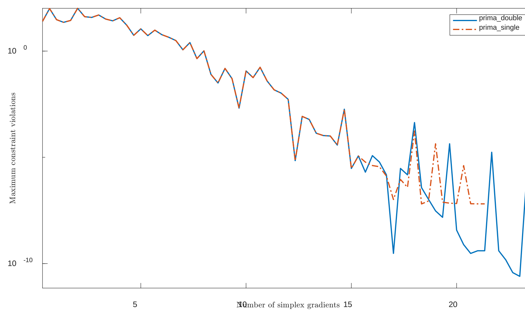
Solving "HS7" with "plain" feature
