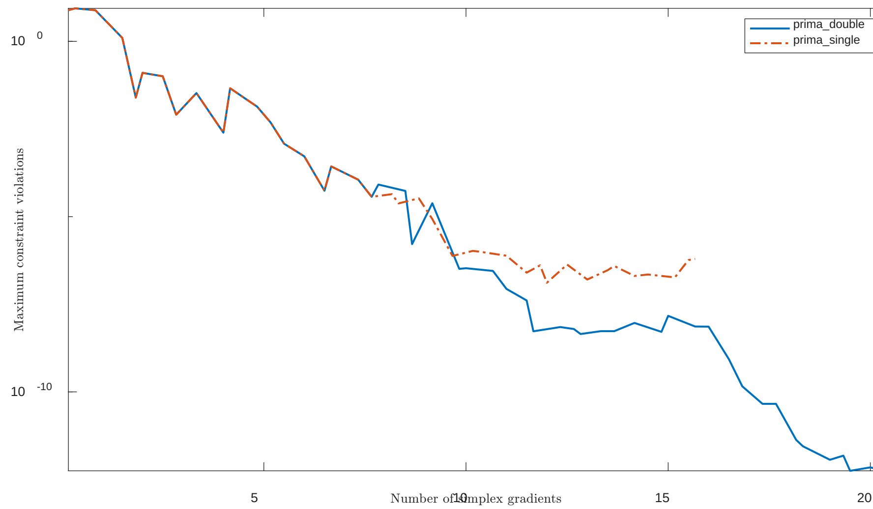
Solving "HS79" with "plain" feature
