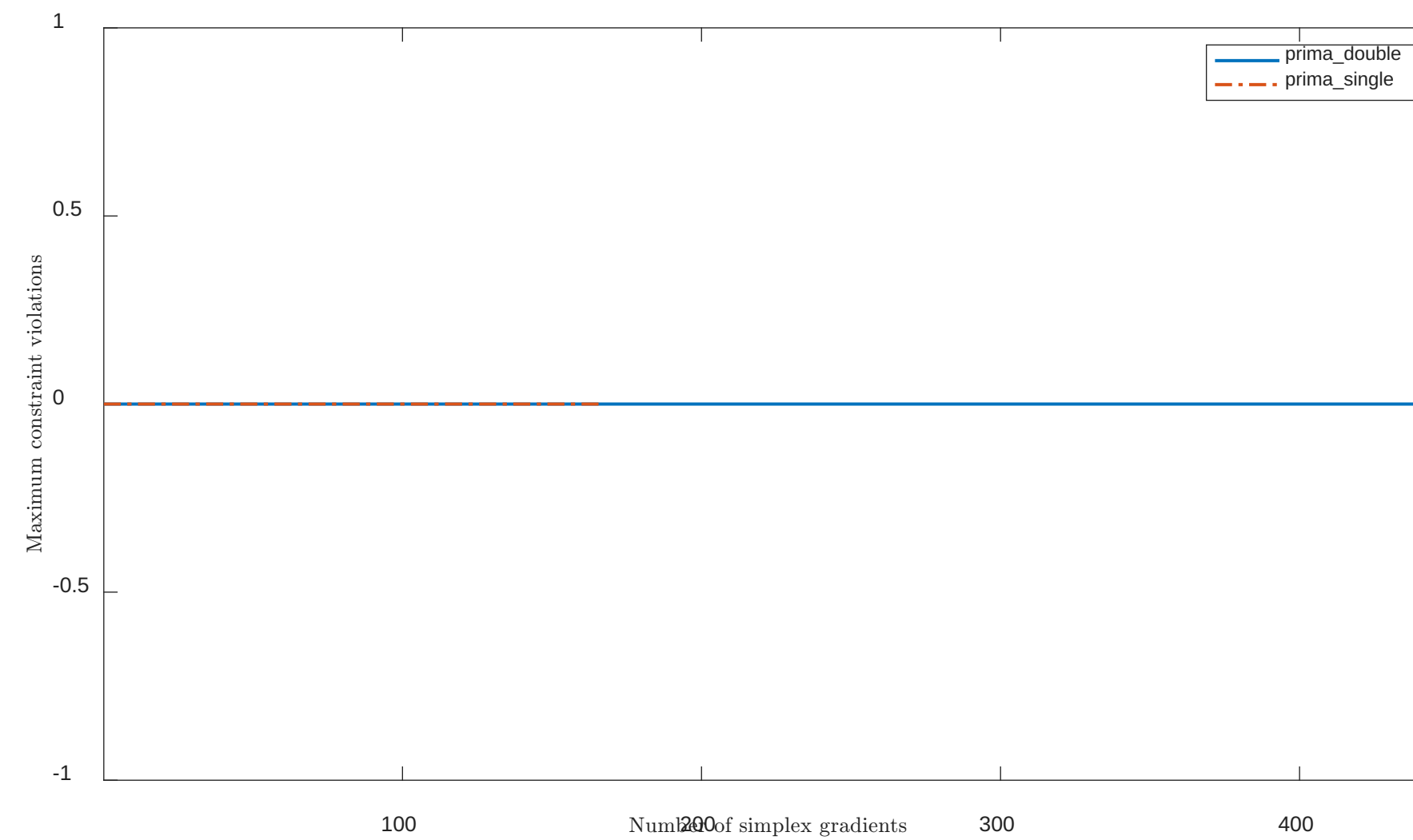
Solving "PALMER3E" with "plain" feature
