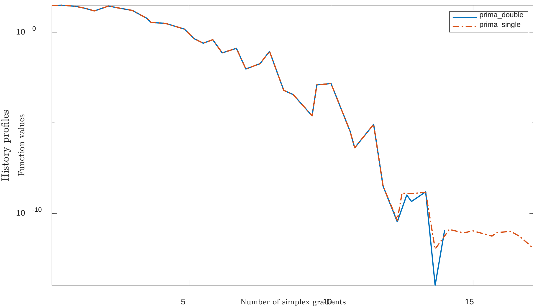
Solving “QING” with “plain” feature
