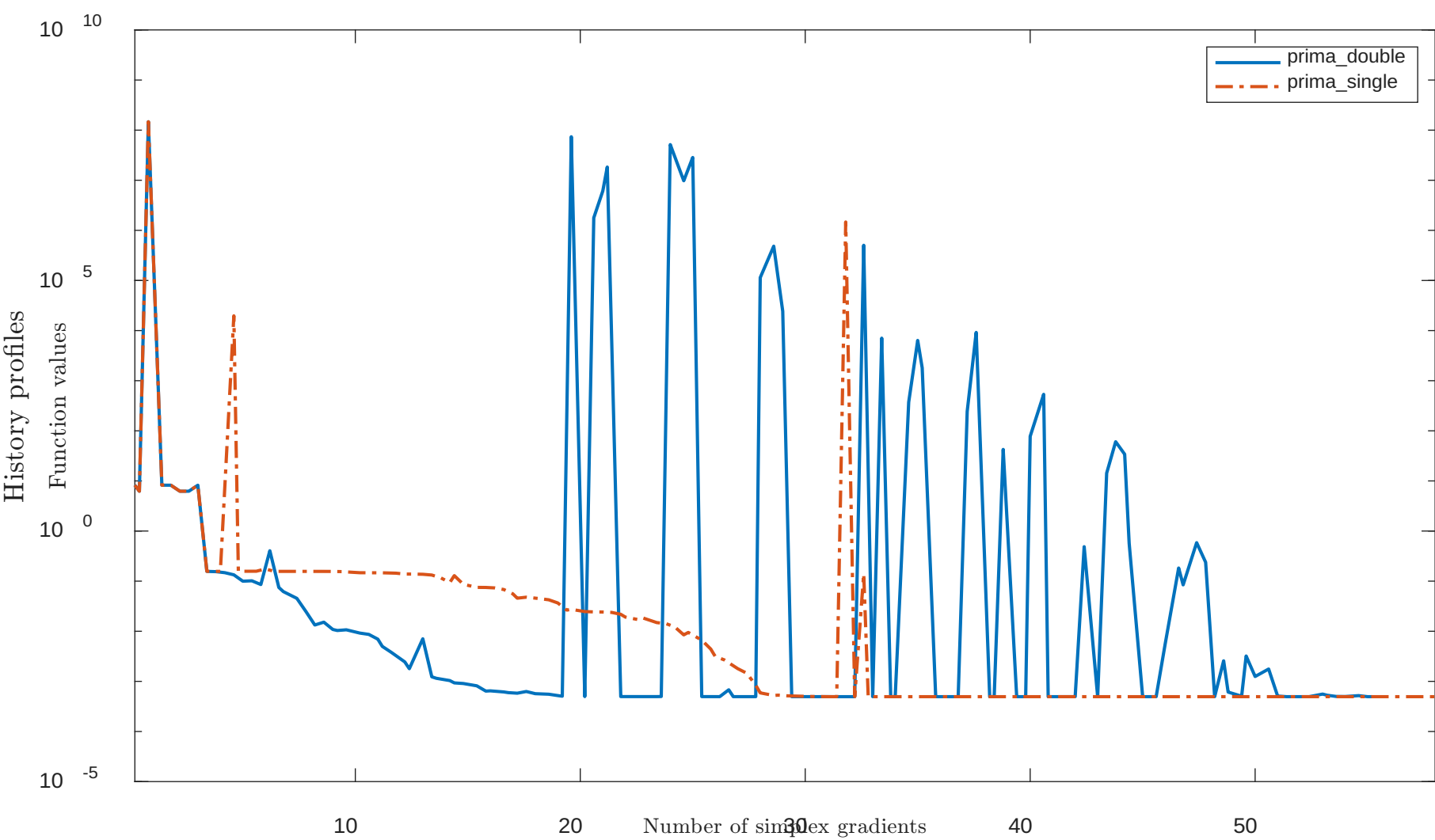
Solving "ROSZMAN1LS" with "plain" feature
