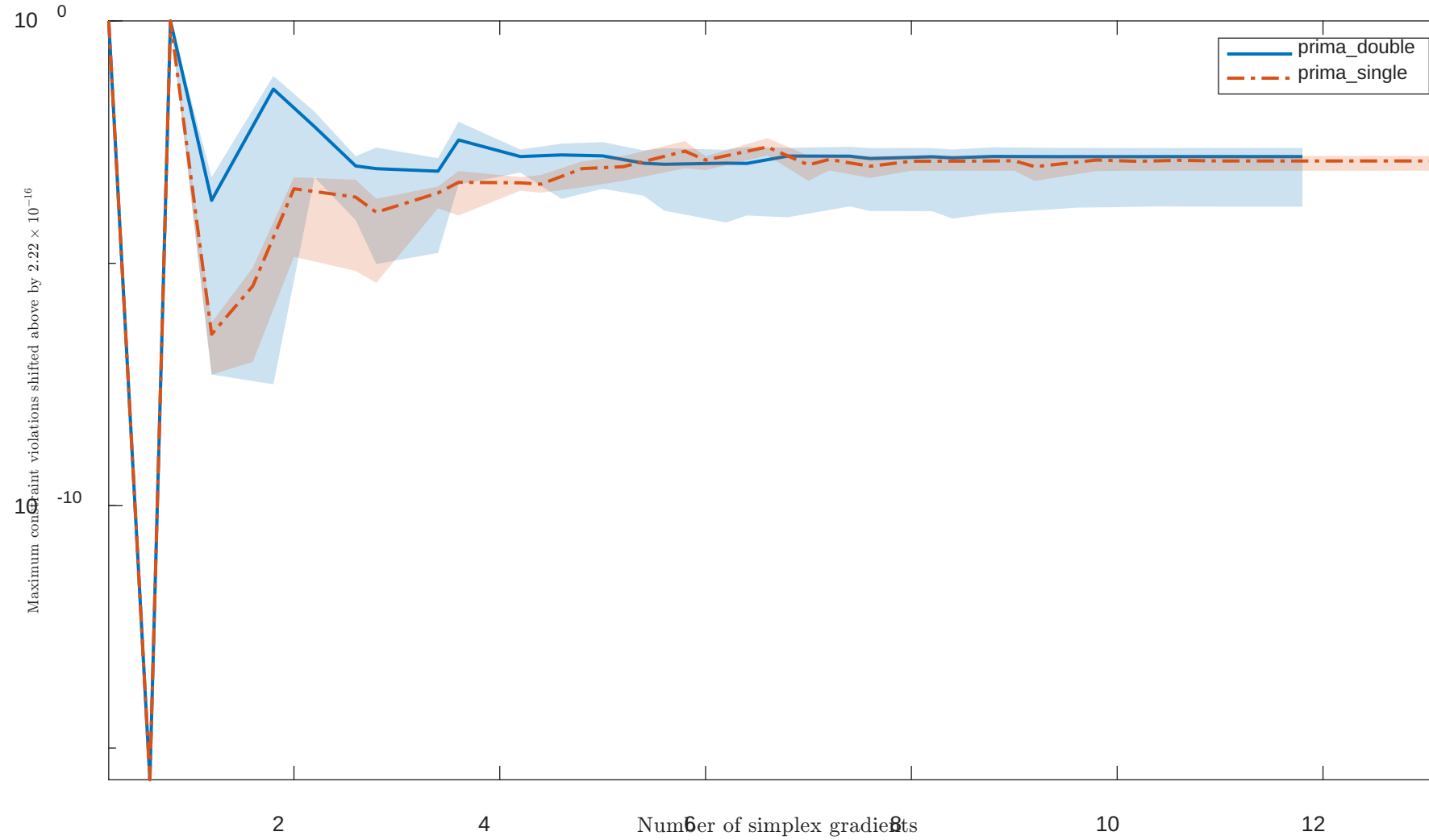
Solving "ALLINITC" with "noisy" feature
