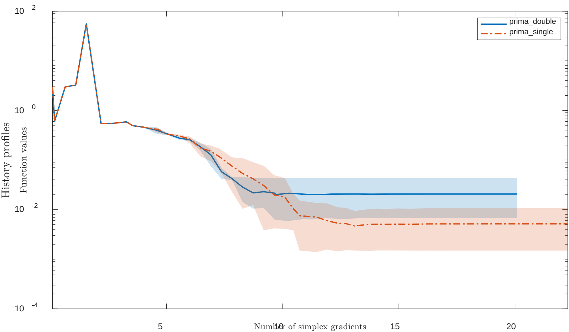
Solving “ARGTRIGLS” with “noisy” feature
