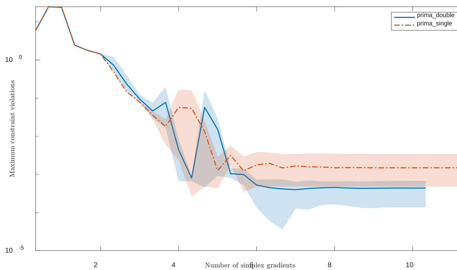
Solving "BT10" with "noisy" feature
