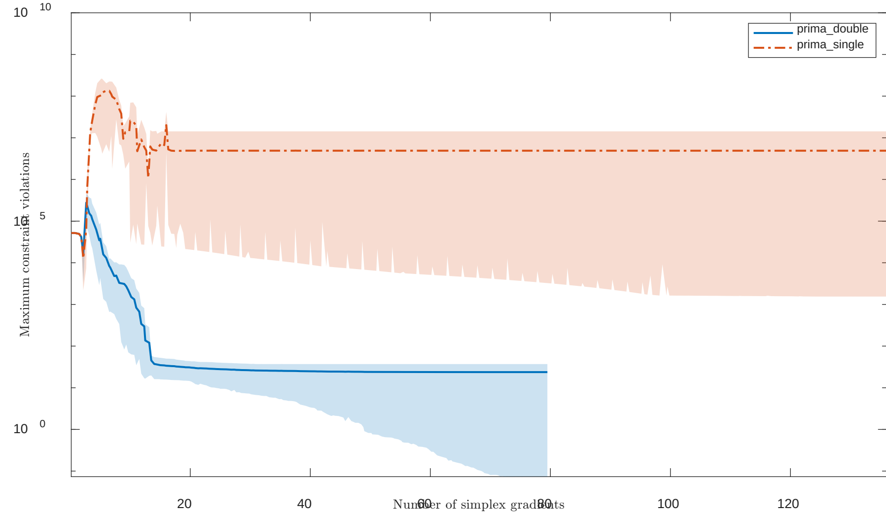
Solving "BT13" with "noisy" feature
