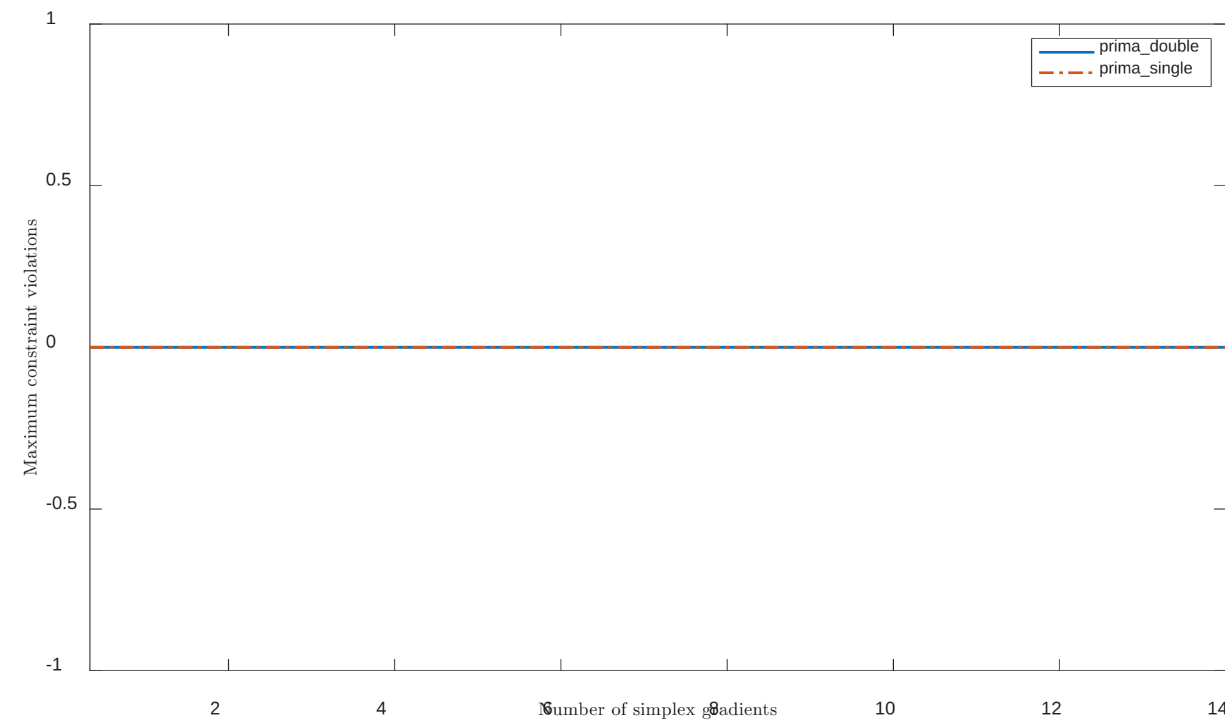
Solving "CAMEL6" with "noisy" feature
