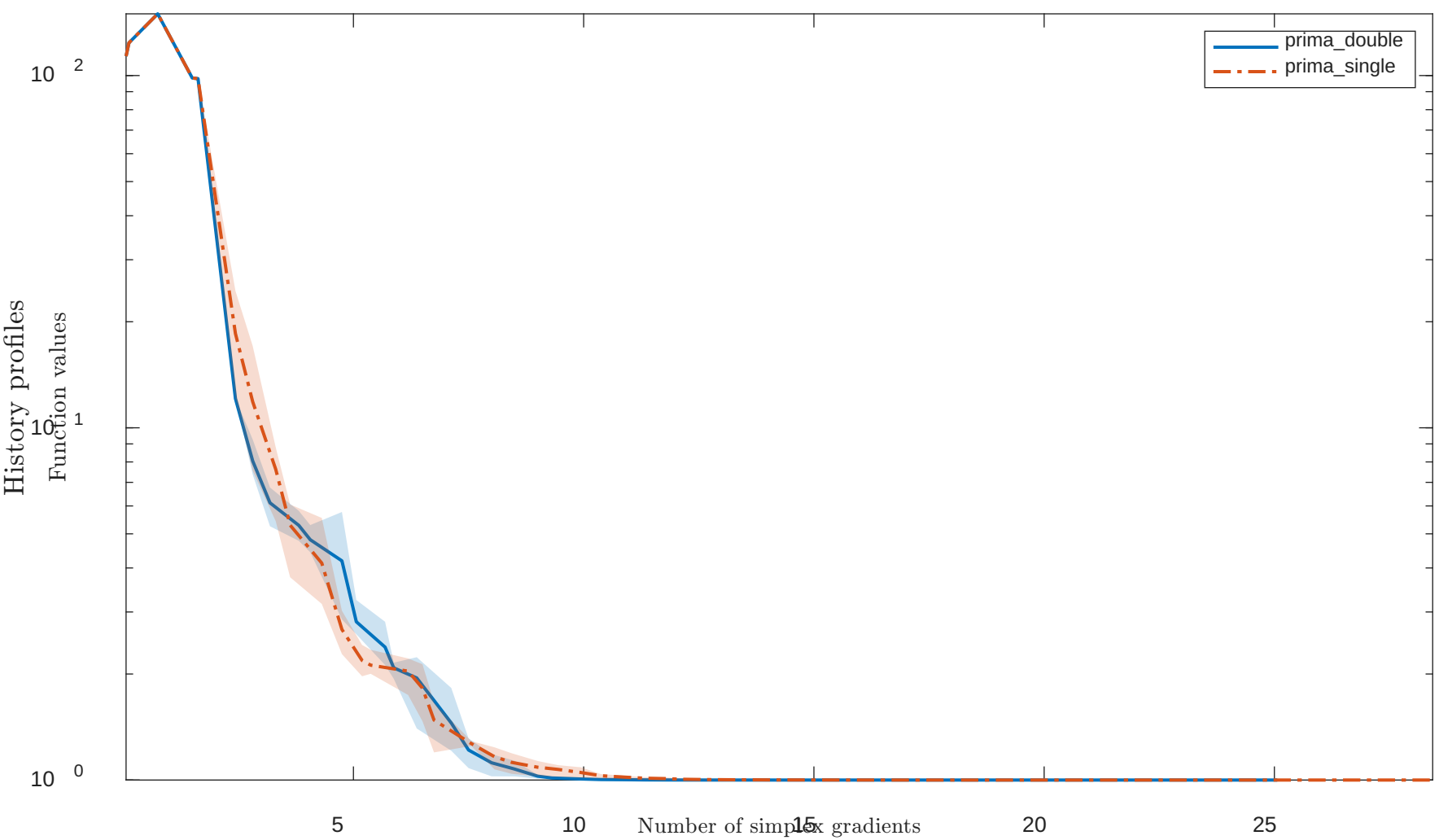
Solving “DIXMAANE1” with “noisy” feature
