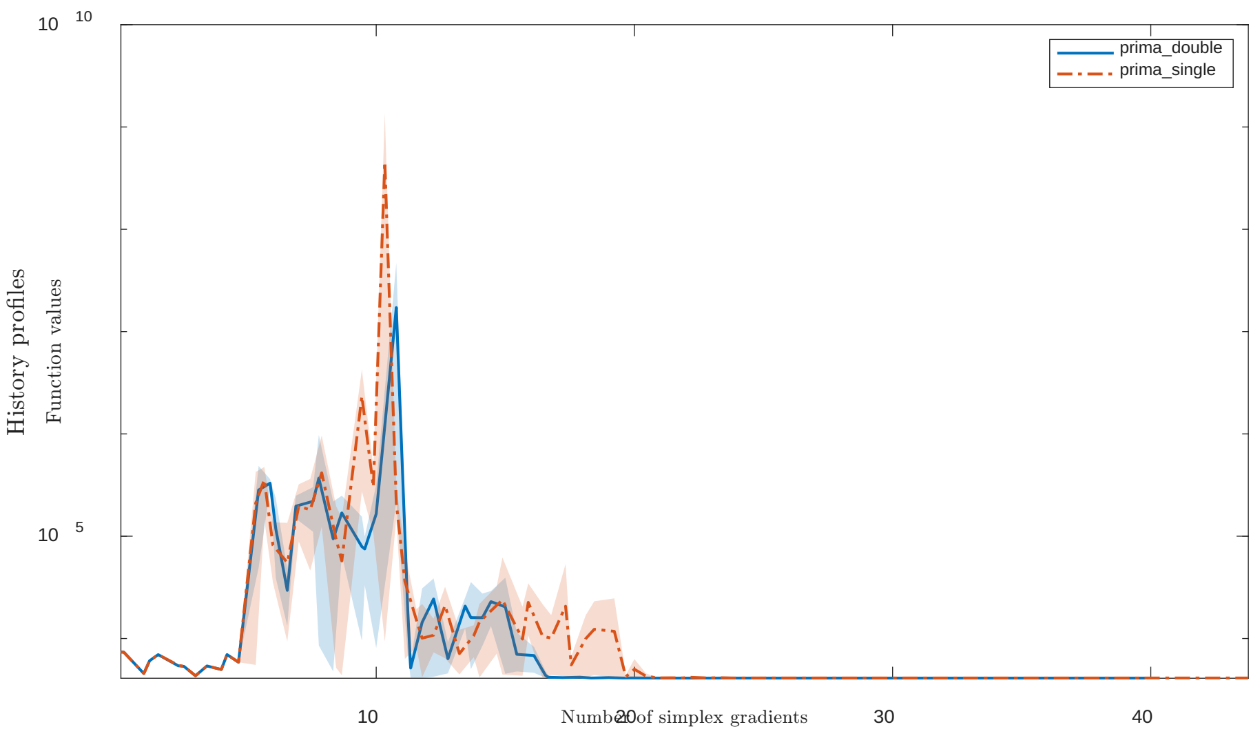
Solving “GAUSS1LS” with “noisy” feature
