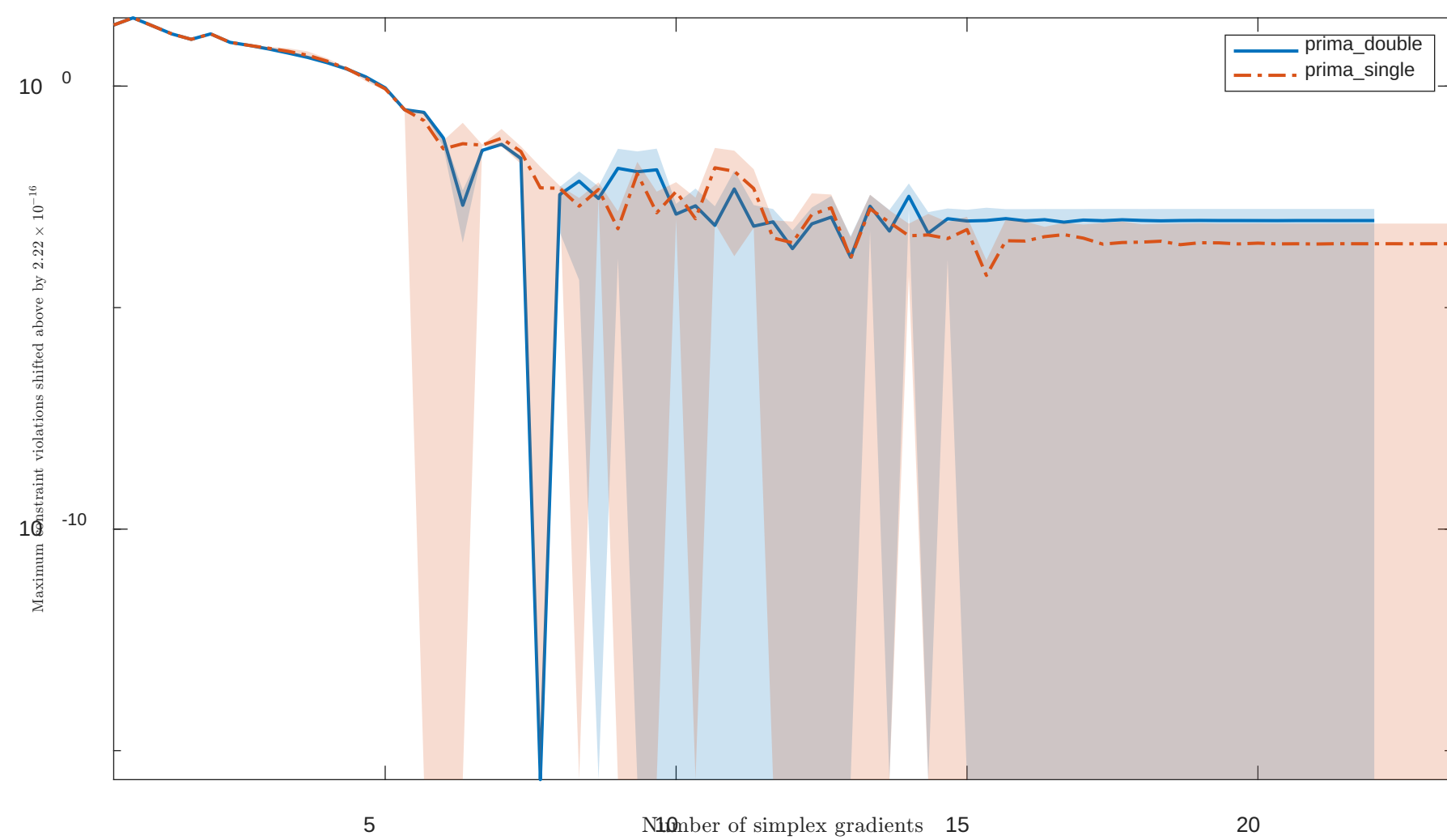
Solving "HS11" with "noisy" feature
