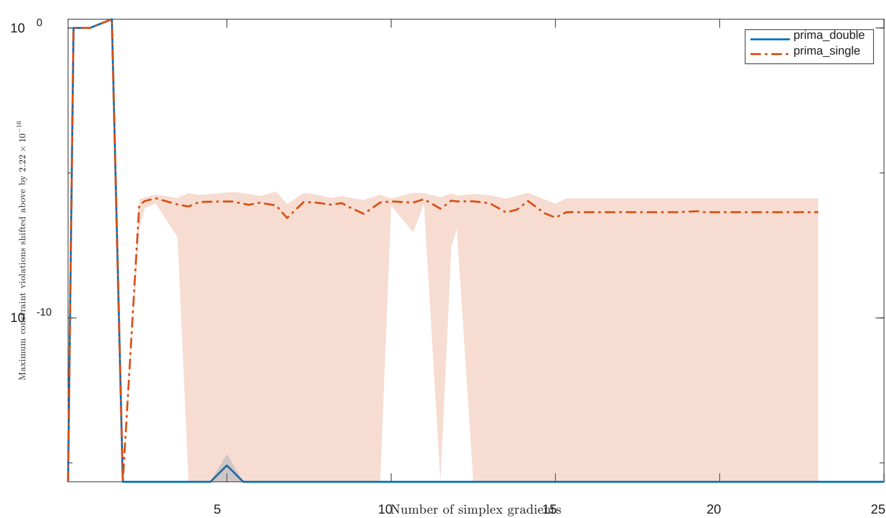
Solving "HS268" with "noisy" feature
