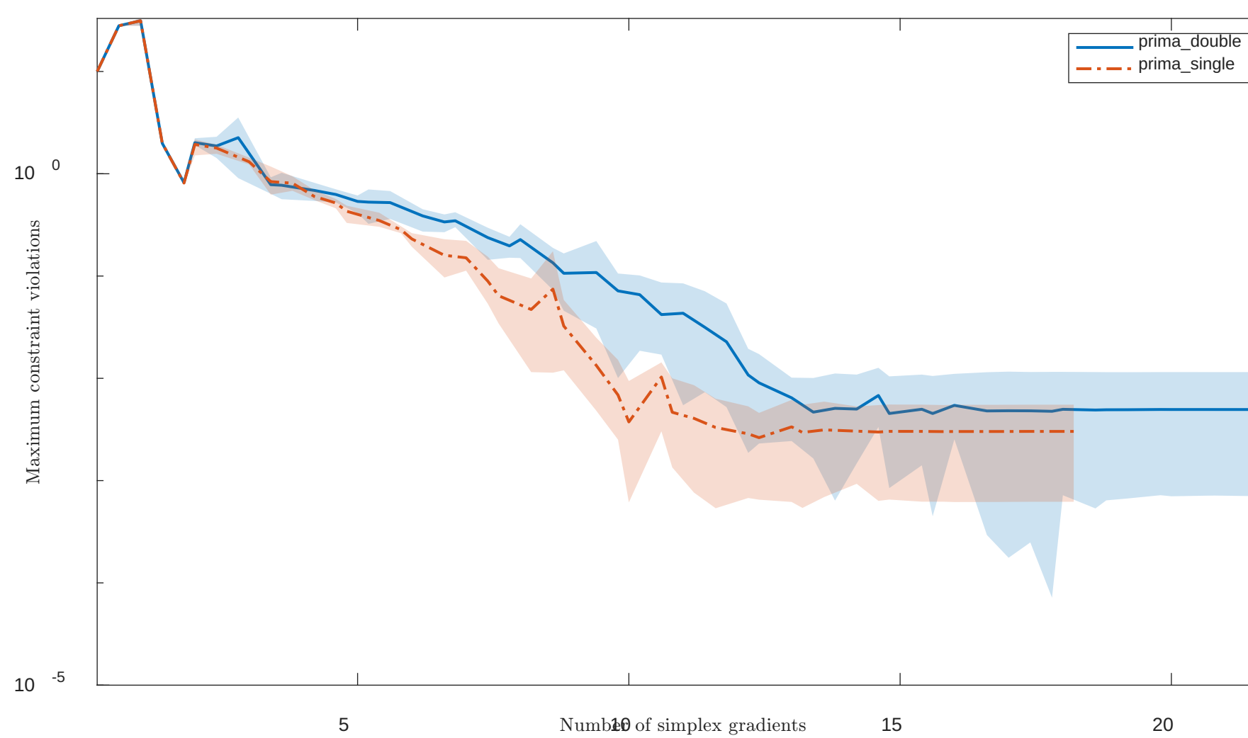
Solving "HS39" with "noisy" feature
