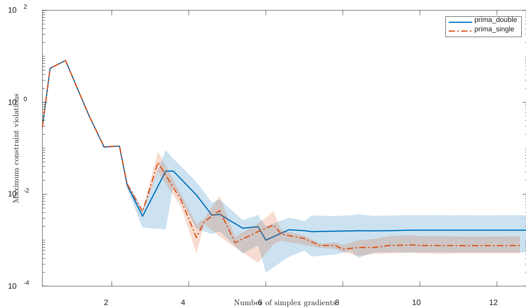
Solving “HS40” with “noisy” feature
