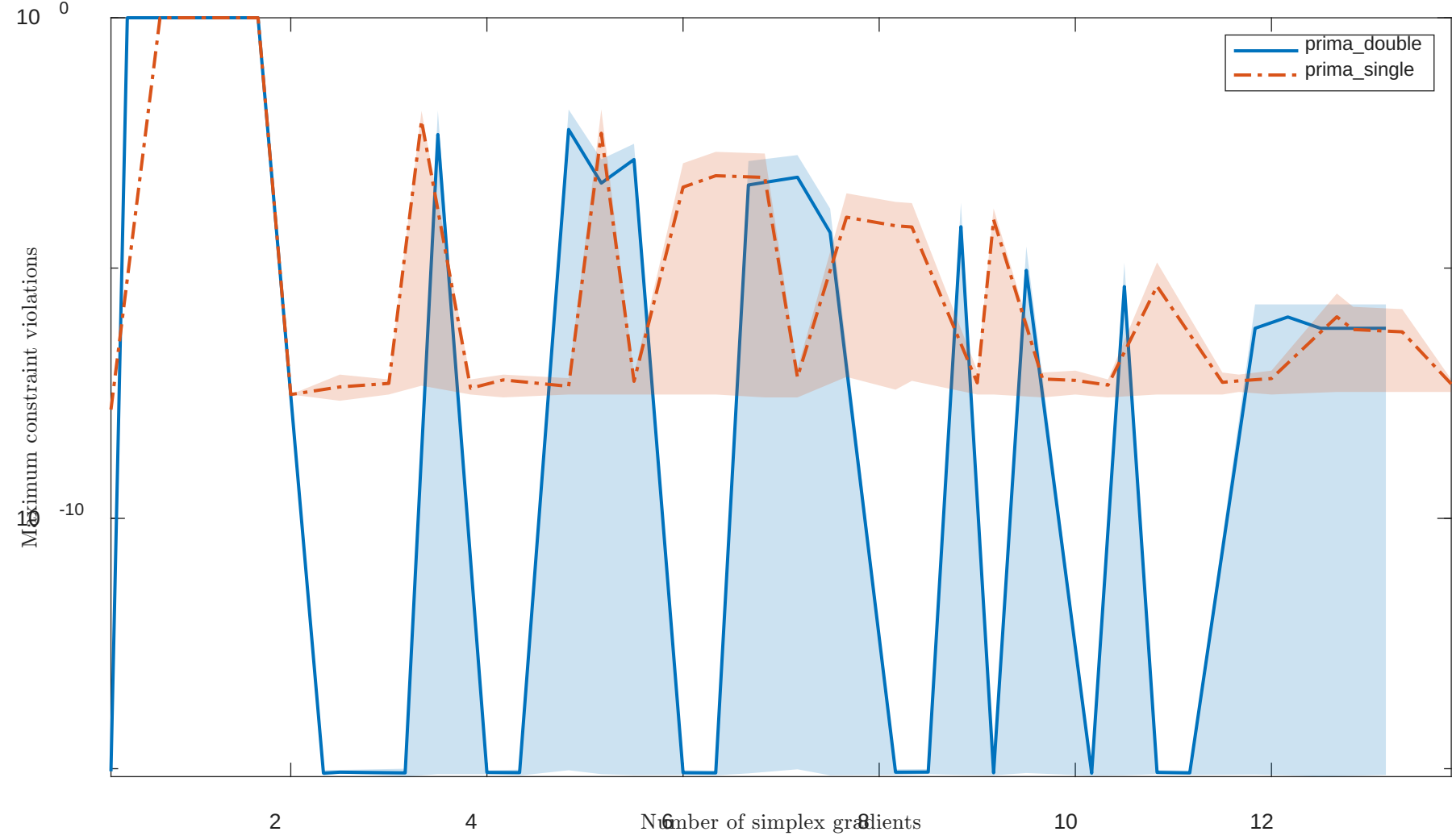
Solving "HS52" with "noisy" feature
