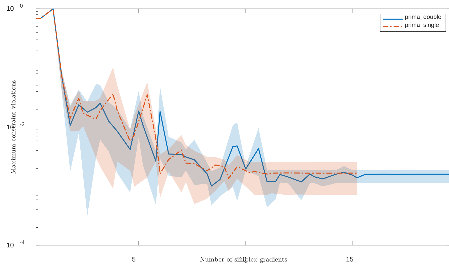
Solving "HS68" with "noisy" feature
