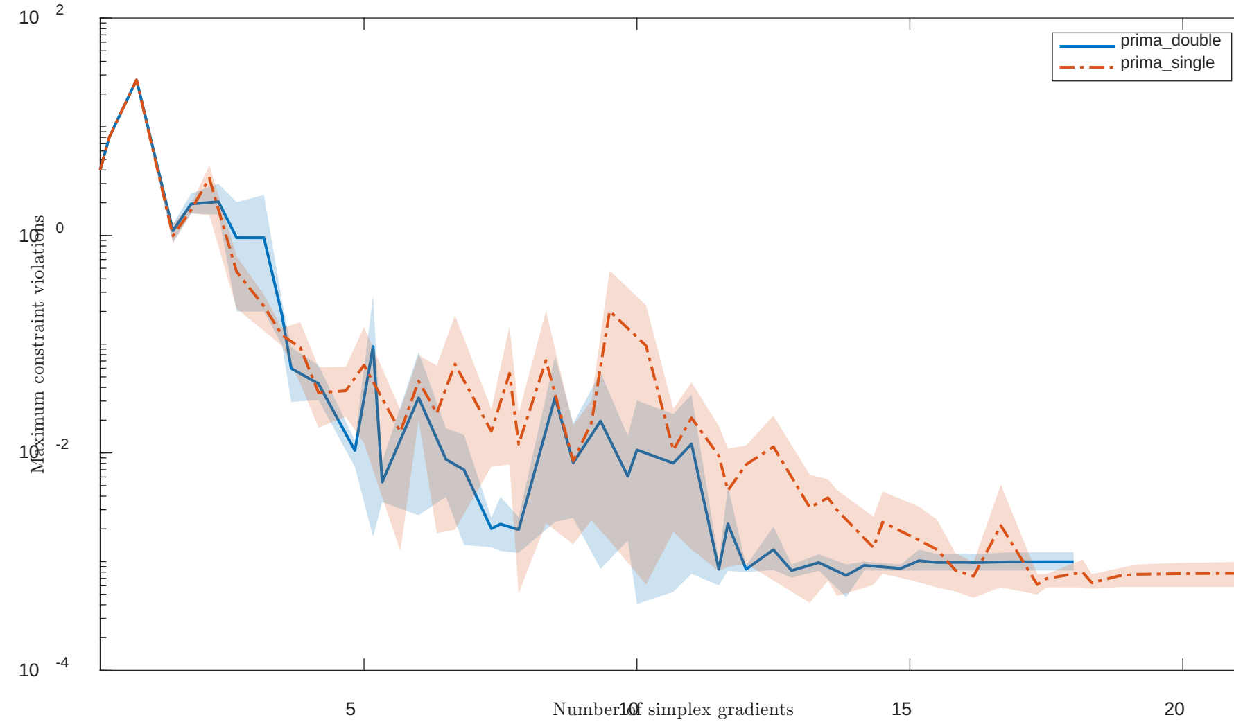
Solving “HS81” with “noisy” feature
