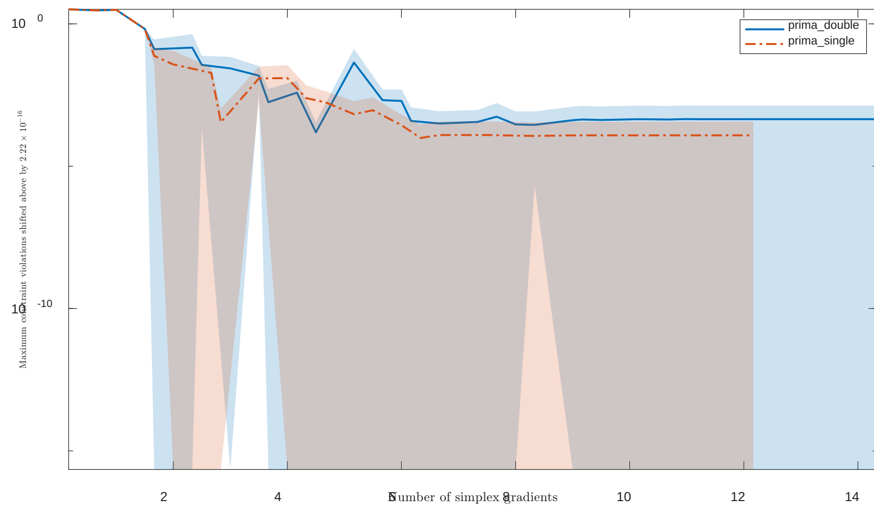
Solving "HS83" with "noisy" feature
