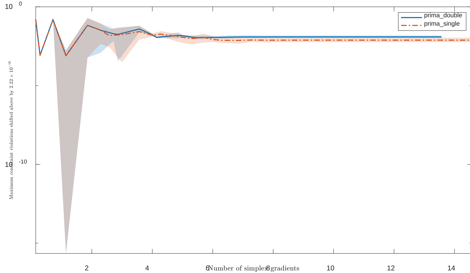
Solving “HS90” with “noisy” feature
