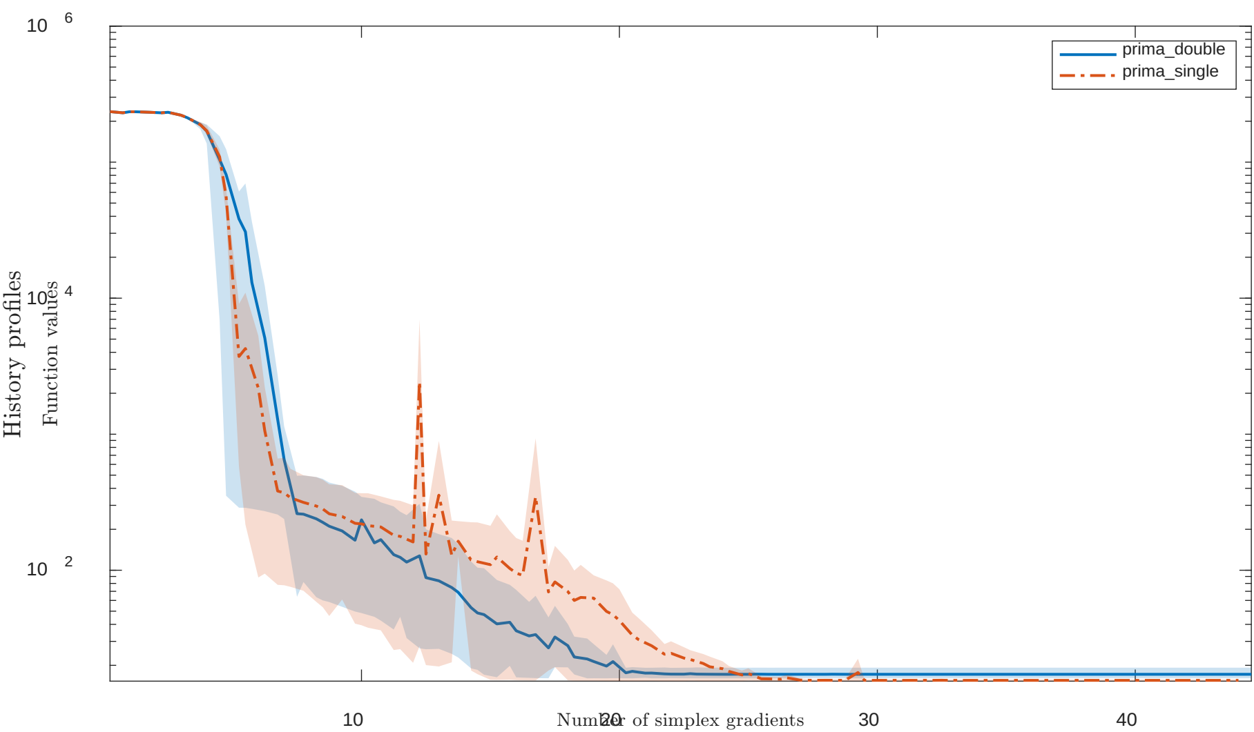
Solving “LSC2LS” with “noisy” feature
