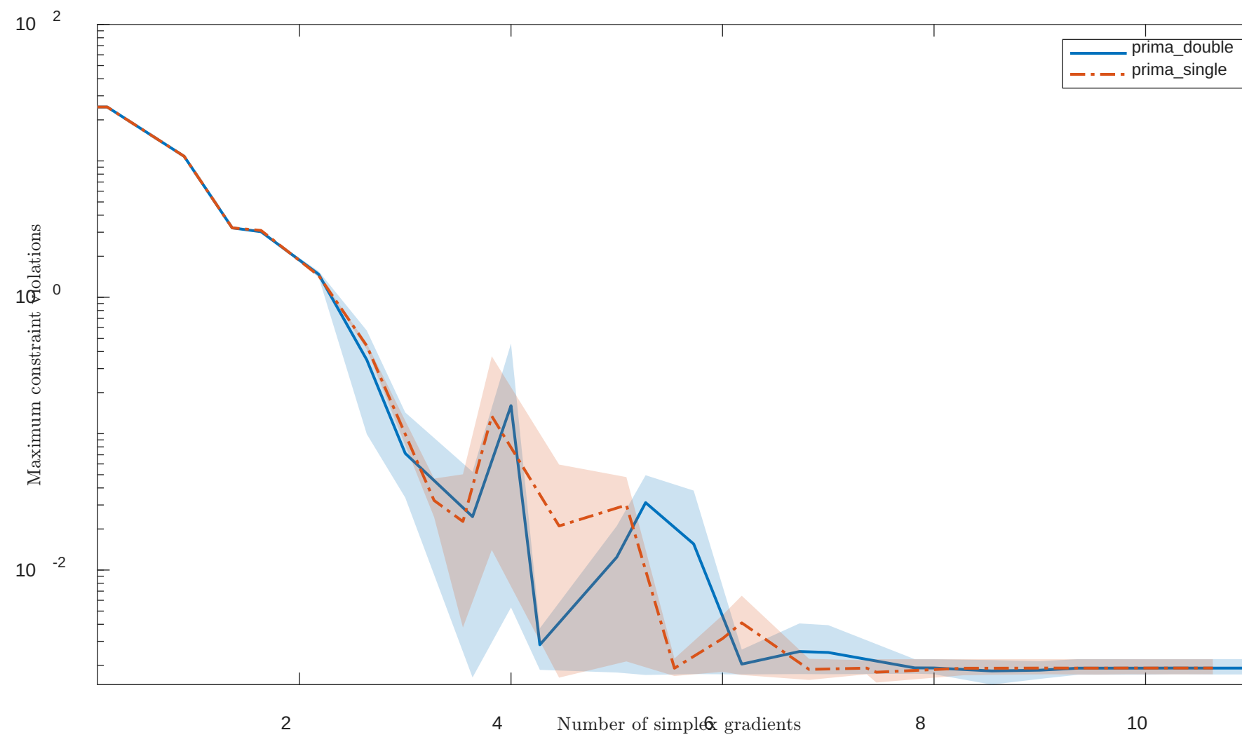
Solving "LUKVLE1" with "noisy" feature
