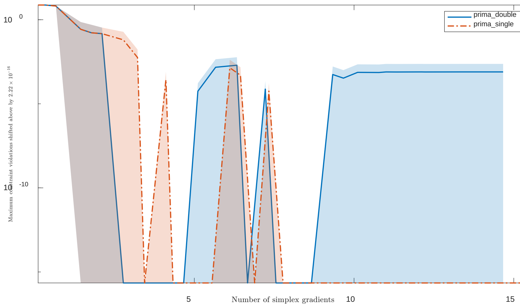
Solving "LUKVLH1" with "noisy" feature
