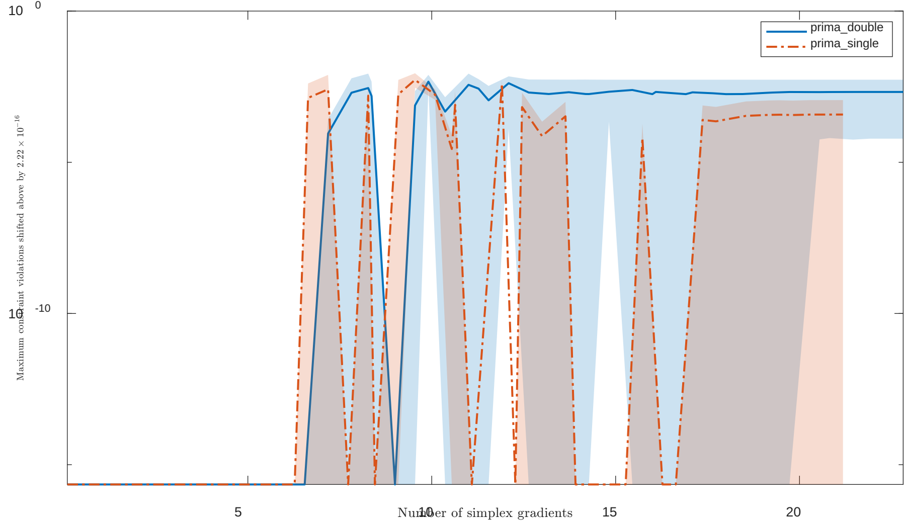
Solving “LUKVL3” with “noisy” feature
