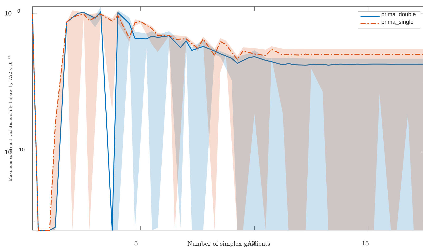
Solving "MAKELA1" with "noisy" feature
