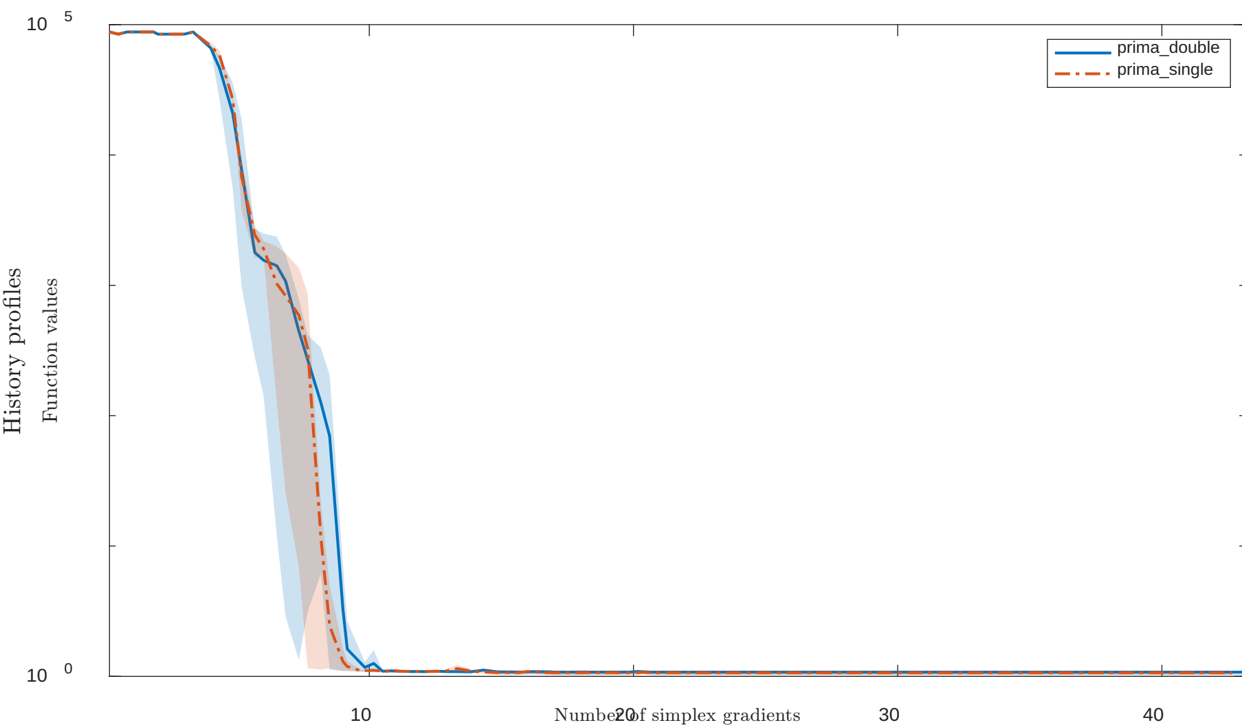
Solving “MGH17SLS” with “noisy” feature
