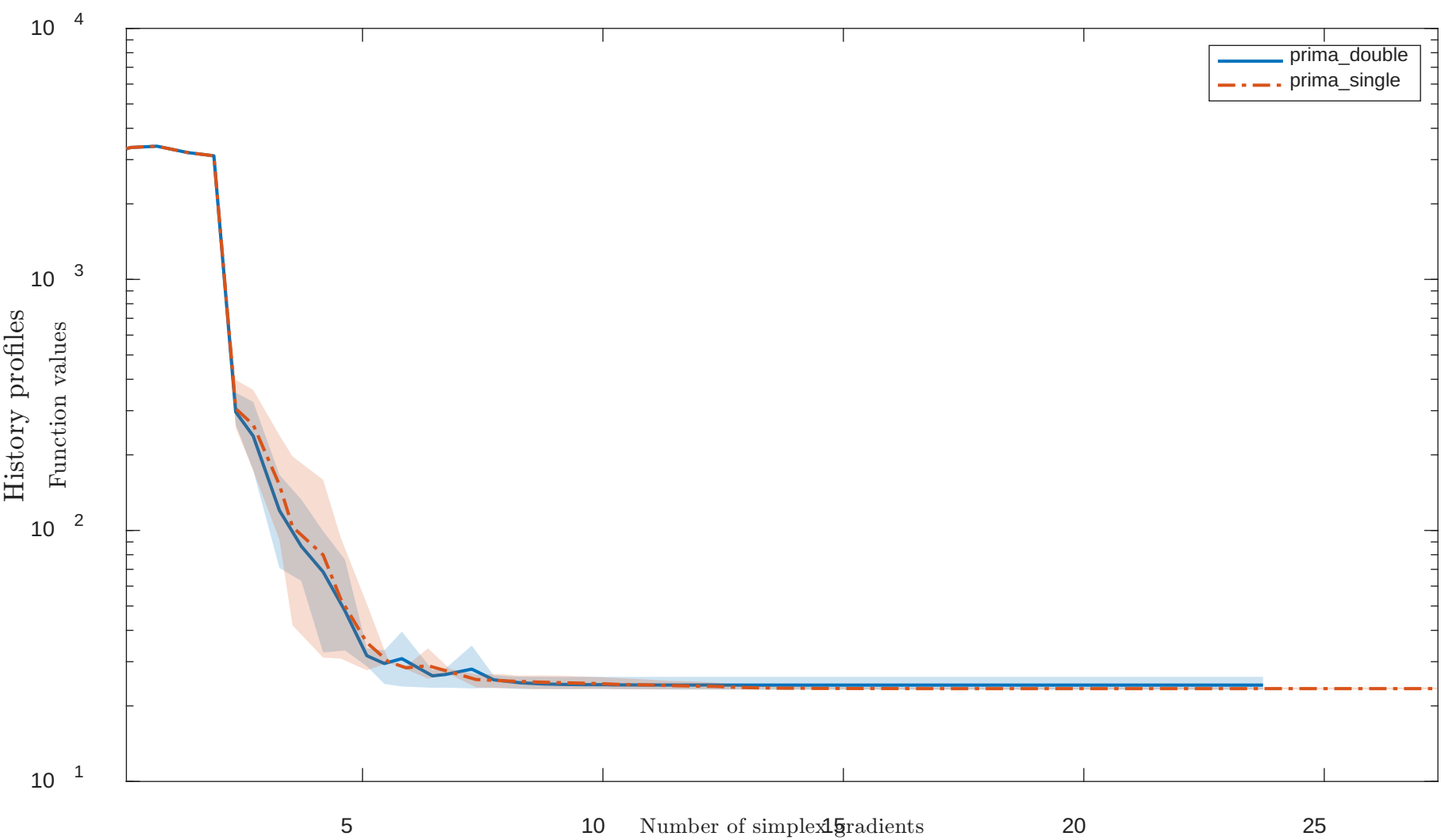
Solving “NONCVXUN” with “noisy” feature
