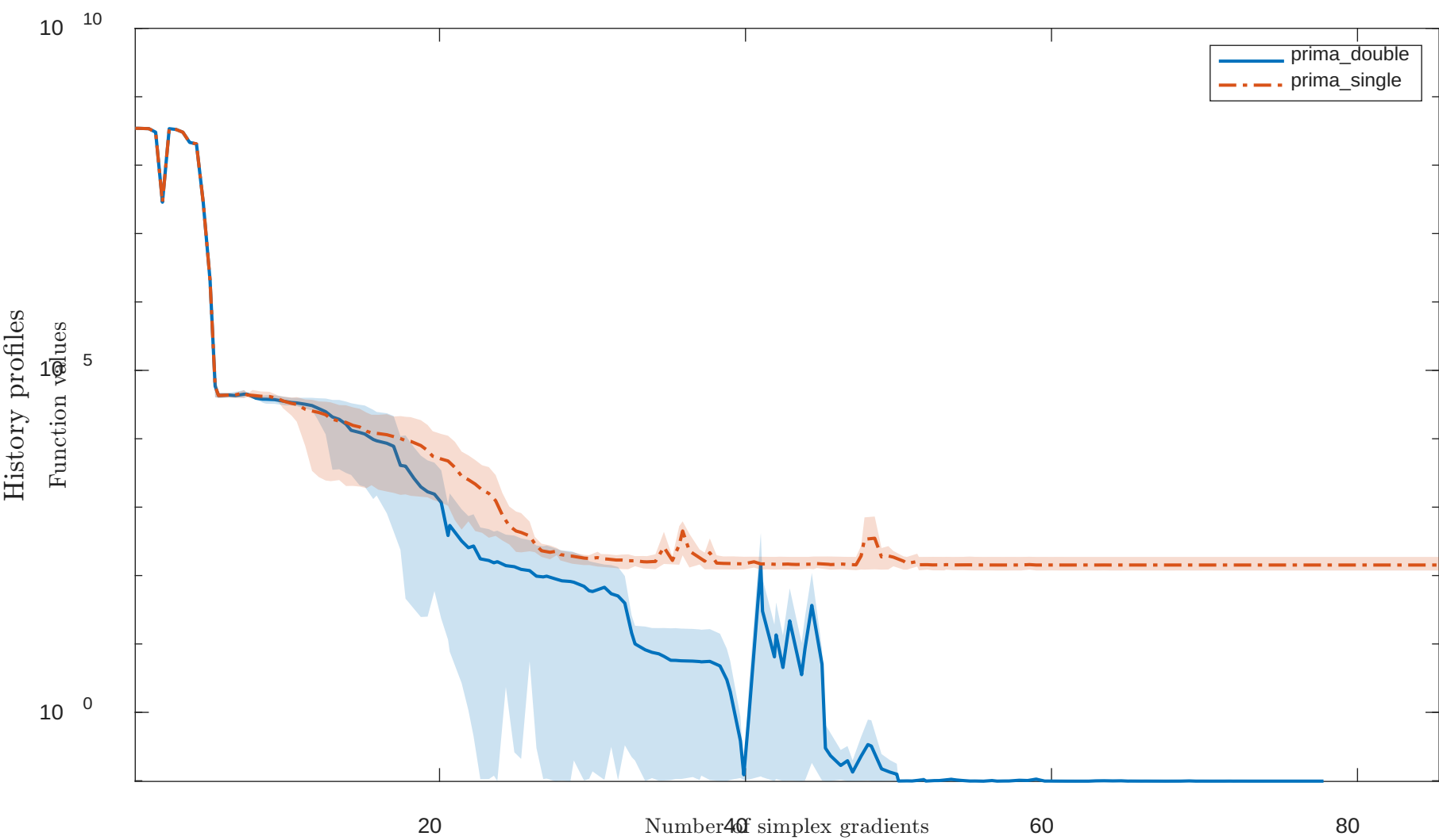
Solving “PALMER1C” with “noisy” feature
