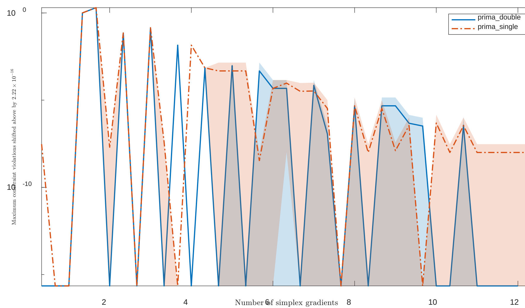
Solving "SIMPLLP" with "noisy" feature
