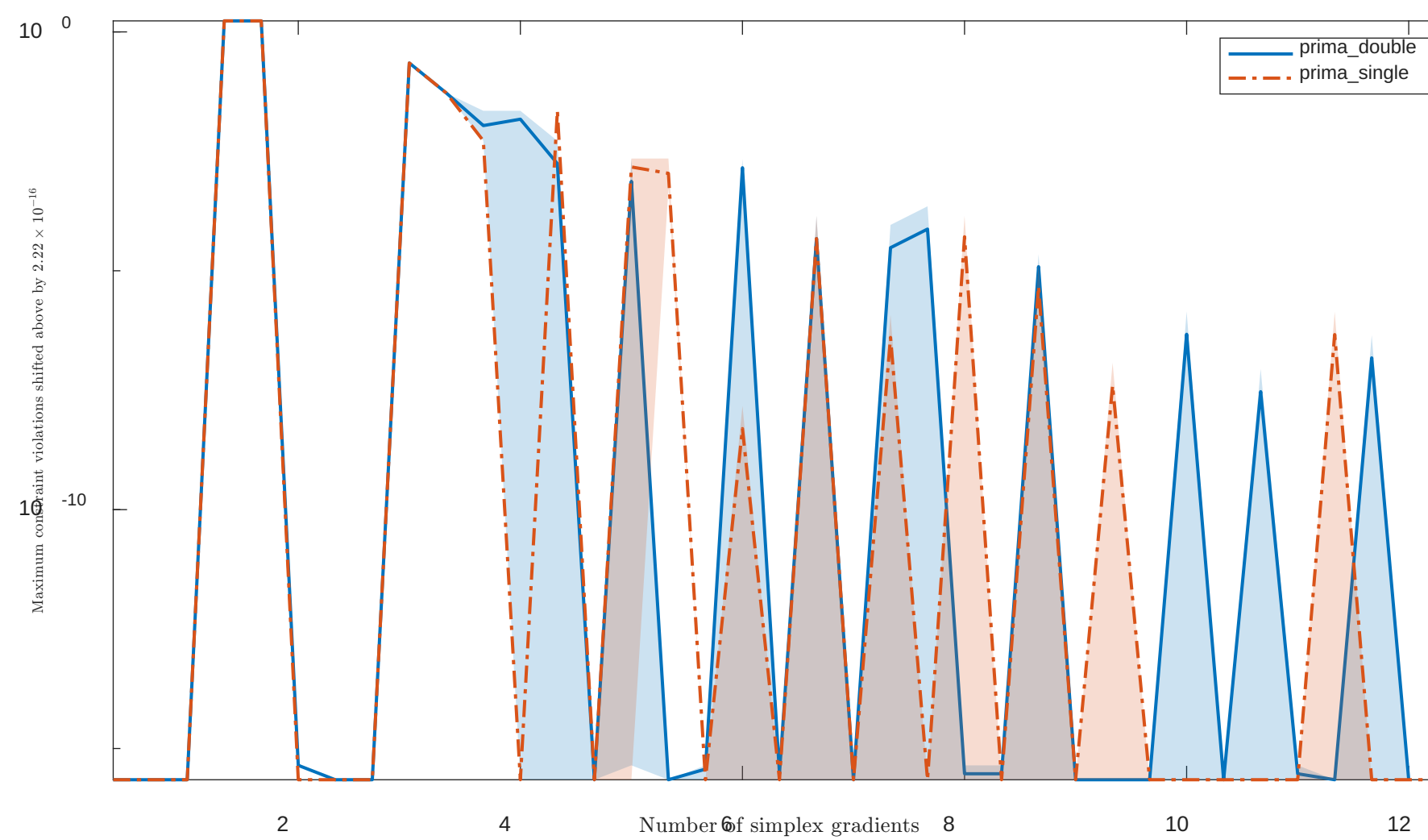
Solving "SIMPLLPB" with "noisy" feature
