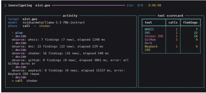
Fig. 4. Live TUI mid-investigation. The activity panel logs each plan/decide/call/observe event; the right panel scores tools exercised so far against findings accumulated.
