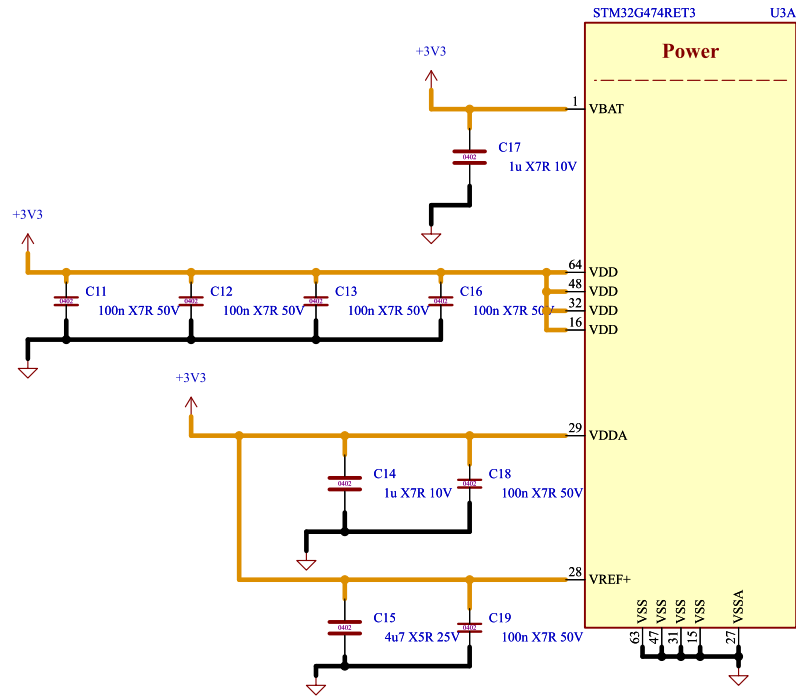
MCU Power Supply Scheme
