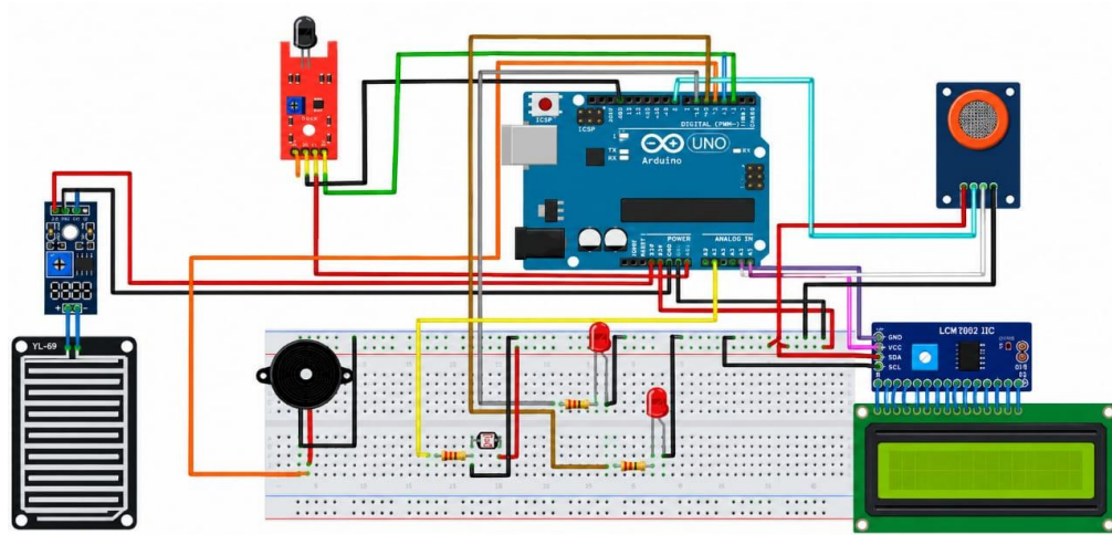
Circuit Diagram
