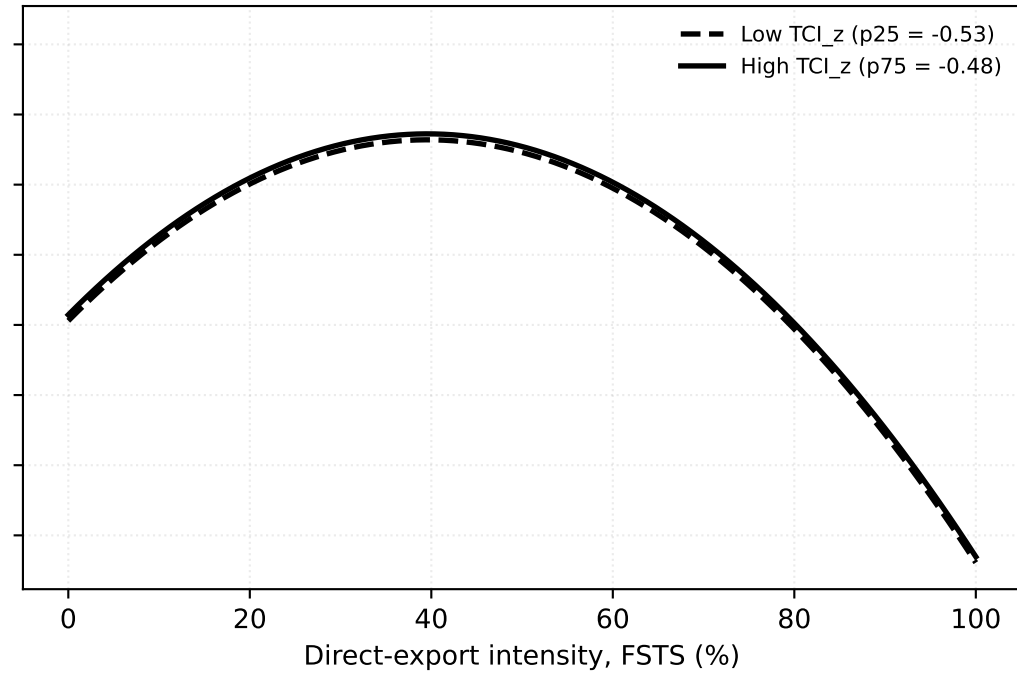
Figure 3b. Predicted \ln(LP) by FSTS at low / high TCI z
