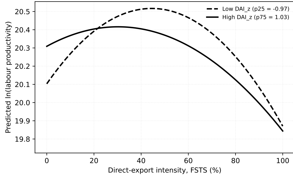
Figure 3a. Predicted \ln(LP) by FSTS at low / high DAI z
