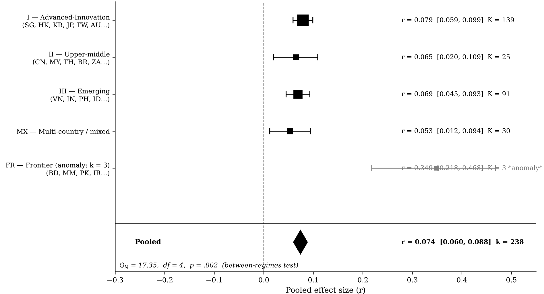
Figure 2. ICRV 5-Regime Subgroup Forest Plot Three-level MARA: k = 238 studies, K = 288 effect sizes
