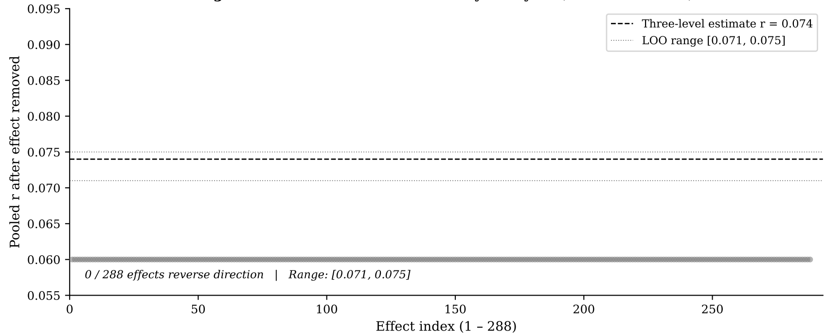
Figure 4. Leave-One-Out Sensitivity Analysis (K = 288 effects)
