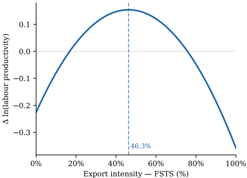
(a) Vietnam 2009 [N = 989]
