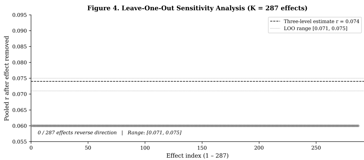
Figure 5: Figure 4: Leave-one-out sensitivity, pooled \bar{r} range across leave-one-out iterations
