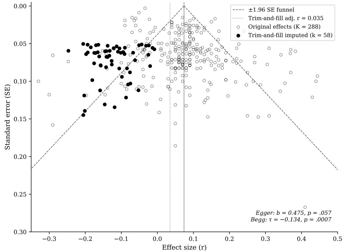
Figure 4. Funnel Plot with Trim-and-Fill Correction k = 58 imputed; adj. r = 0.035 [0.023, 0.048]
