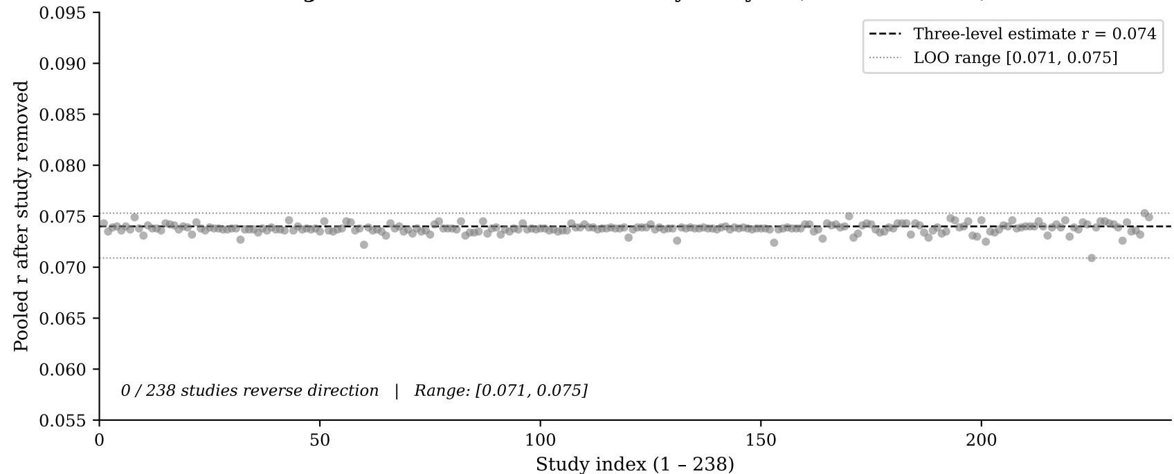
Figure 4. Leave-One-Out Sensitivity Analysis (k = 238 studies)
