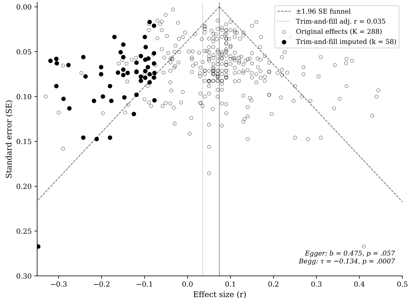
Figure 5. Funnel Plot with Trim-and-Fill Correction k = 58 imputed; adj. r = 0.035 [0.019, 0.051]
