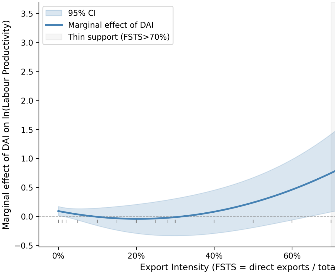
Figure 2: Marginal Effect of DAI across Export Singapore WBES 2023, M8 OLS-HC1 (N=
