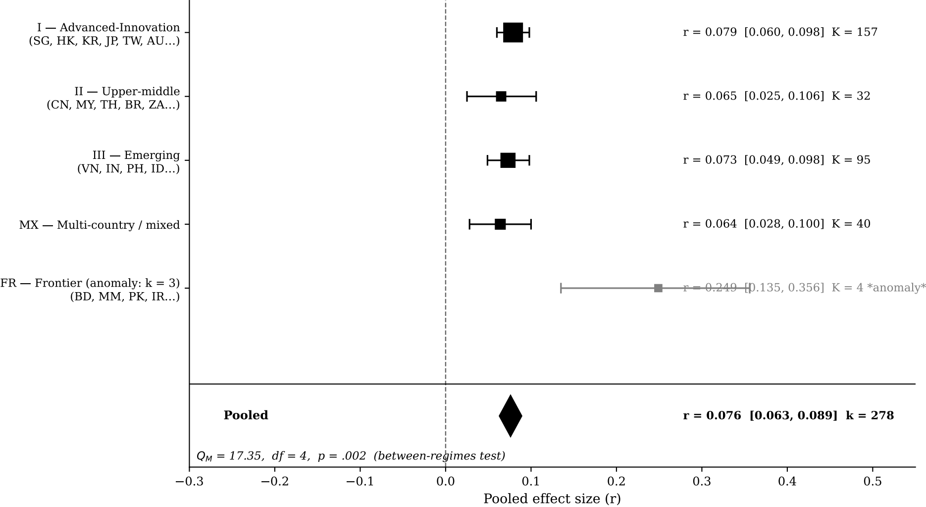
Figure 2. ICRV 5-Regime Subgroup Forest Plot Three-level MARA: k = 278 studies, K = 328 effect sizes
