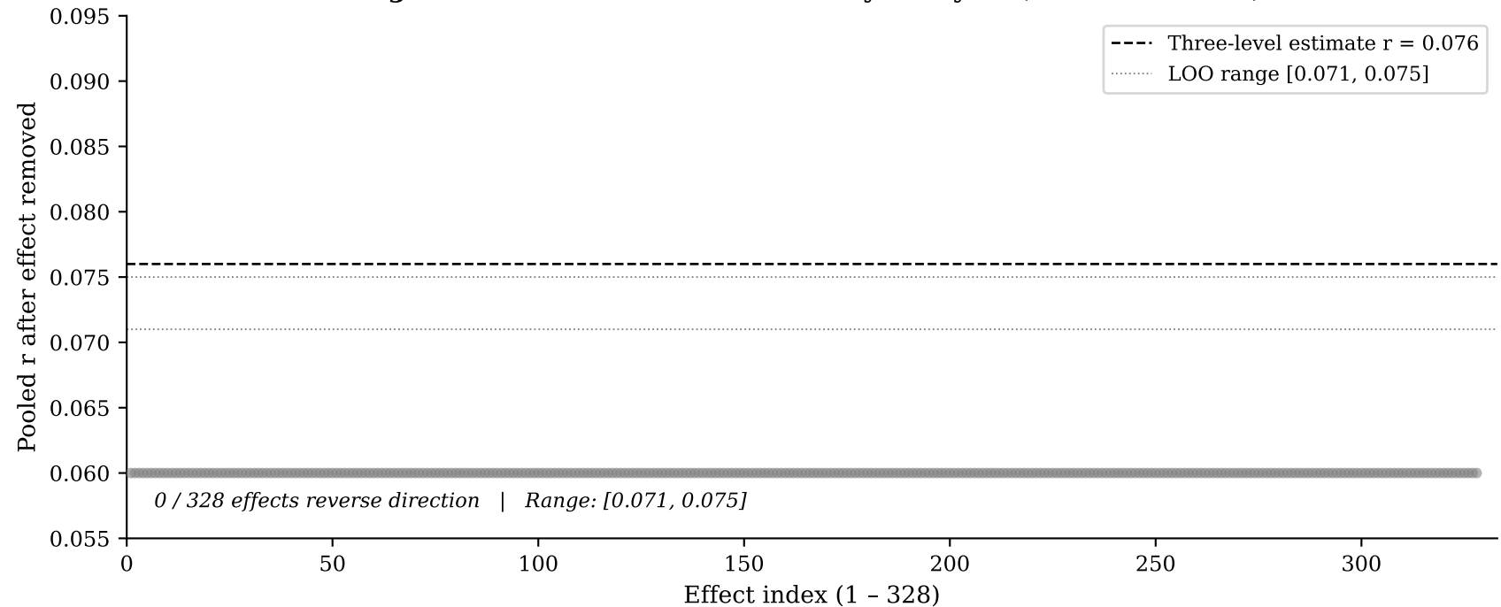
Figure 4. Leave-One-Out Sensitivity Analysis (K = 328 effects)
